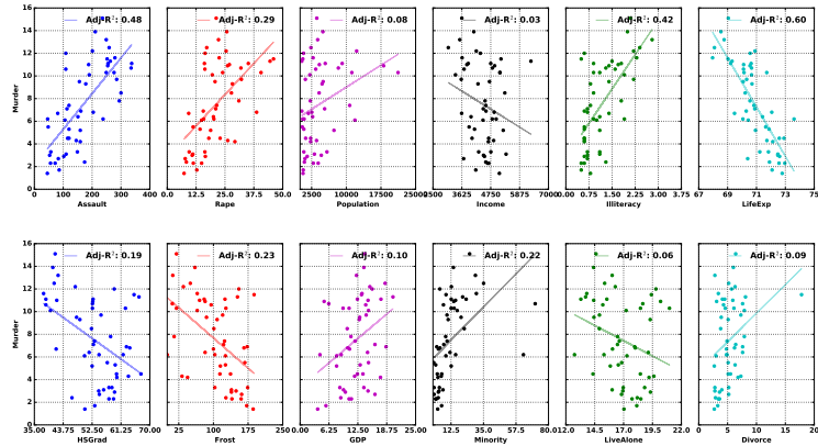
Figure 3: Pairwise regression of murder on various state predictors. Assault, Rape, LifeExp, and Minority appear correlated with murder rates, where simple linear regression accounting for over 20% of the variation. The relationship is clearly non-linear for other predictors, such as Population and Divorce rates.
