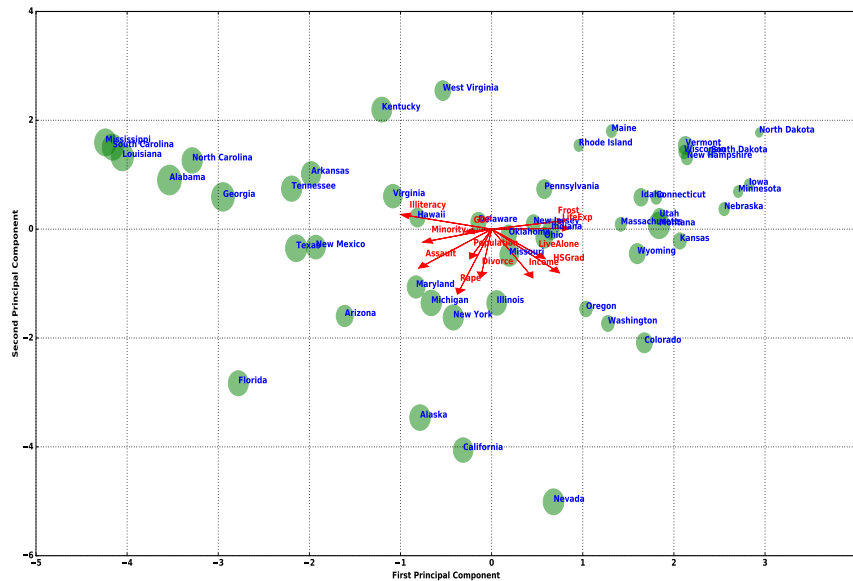
Figure 4: Principal component analysis of the feature matrix. Each circle represents the projection of the state onto the 2-dimensional plane spanned by the first and second principal components. The size of the circle is proportional to the murder rate. The projection of the variables themselves are shown in red and indicate the contribution of each variable to the first and second PCs. The columns are clustered into roughly four groups: (Forst, LifeExp), (LiveAlone, HSGrad, Income), (Rape, Divorce, Population, Assault), and (GDP, Minority, Illiteracy).
