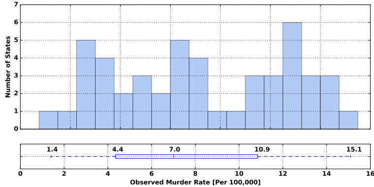
Figure 2: Histogram and boxplot of the murder rates. The histogram suggest the marginal distribution of murder rates is multi-modal. The boxplot shows a right skew in the data, which indicates that there is greater variability at higher values in the murder distribution
