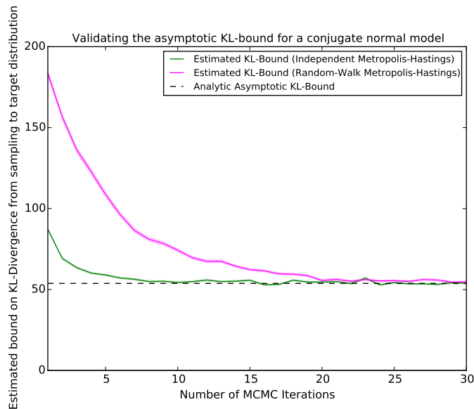
Figure 1: Validation of Algorithm 3.6.1 applied to a conjugate normal model ( \mu_0 = 0, \sigma_0 = 10, \sigma = 1 ) using an independent Metropolis-Hastings (IMH) with proposal from the prior, and a random-walk Metropolis Hastings with a \mathcal{N}(\mu, 2) proposal.
